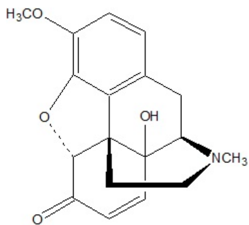
14-Hydroxycodeinone
